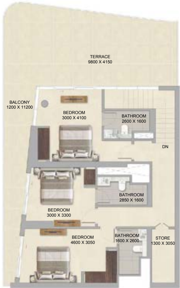
UPPER LEVEL
