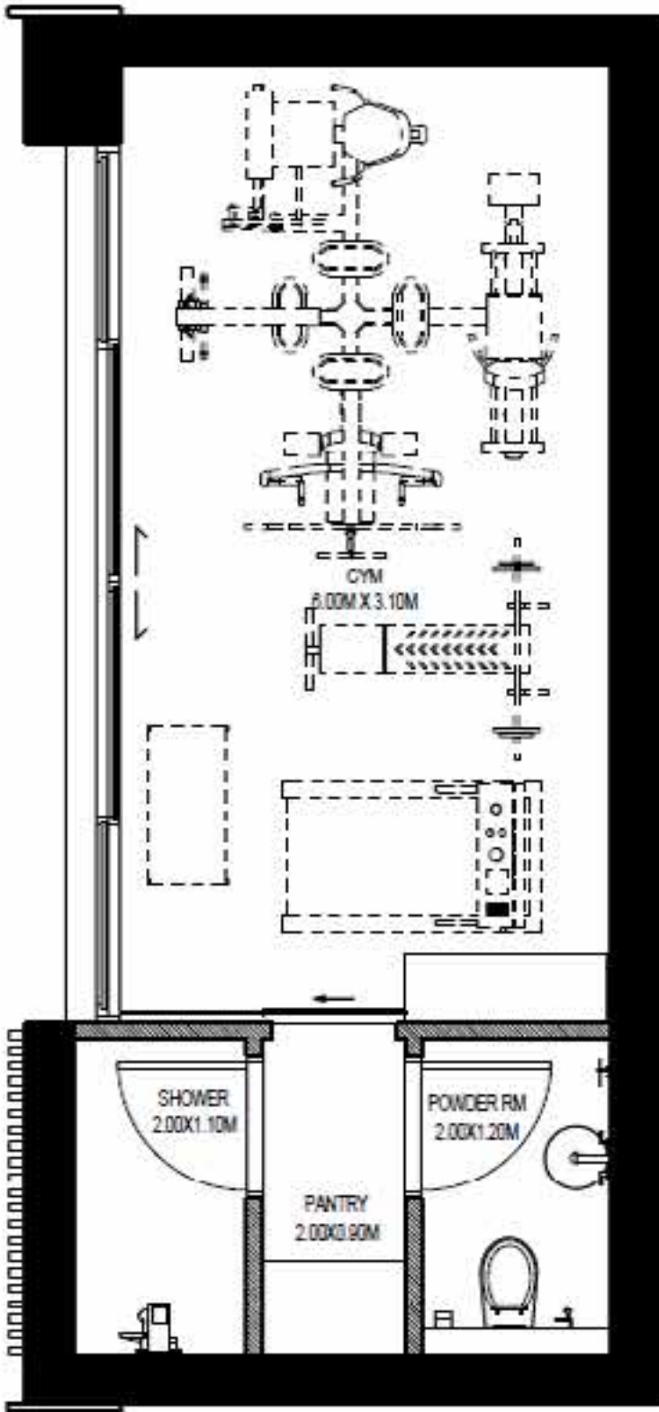
GYM LAYOUT
